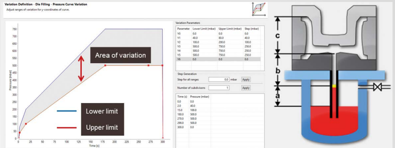
Assistants for fast and easy estimation of pressure conditions for filling the stalk, casting and cavity
