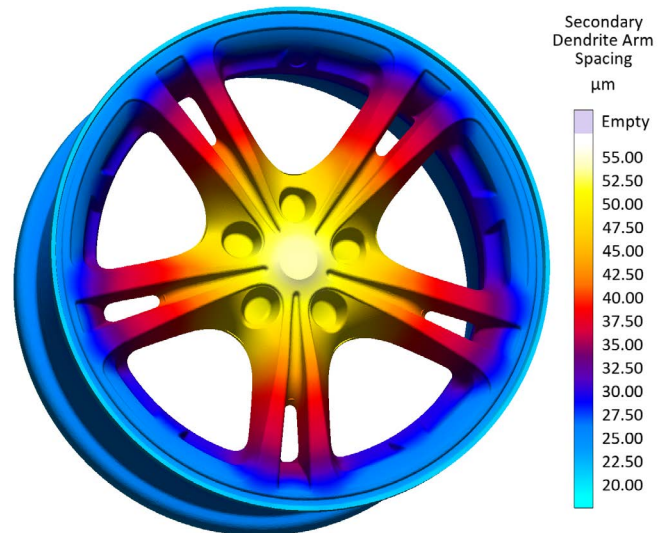
Calculated local secondary dendrite arm spacing
